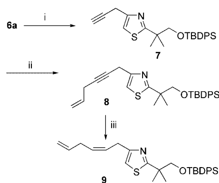
(Z) model: Wittig approach
