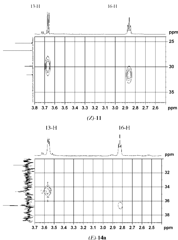
Figure 1. Edited gHSQC experiment of models 11 (in \text{CDCl}_3 ) and 14a (in \text{C}_6\text{D}_6 ).
