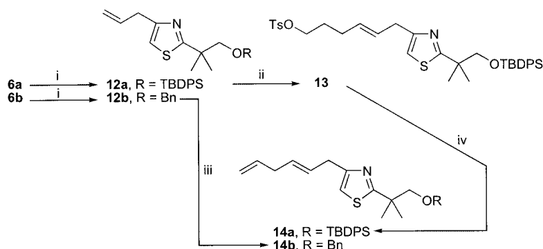
Scheme 4. Synthesis of analogs of mycothiazole with a ( E )- \Delta^{14} configuration. Reagents and conditions: (i): \text{InCl}_3 , \text{CH}_2=\text{CHMgBr} , \text{Pd}(\text{dppf})\text{Cl}_2 , THF, 80%; (ii): \text{CH}_2=\text{CHCH}_2\text{CH}_2\text{CH}_2\text{OTs} , Grubbs 2nd generation, catalyst, PhMe, 80 °C, 50%. (iii): \text{CH}_2=\text{CHCH}_2\text{CH}=\text{CH}_2 , Grubbs 2nd generation, \text{CH}_2\text{Cl}_2 , room temp., 20%. (iv): NaI, DBU, DME, 20%.
