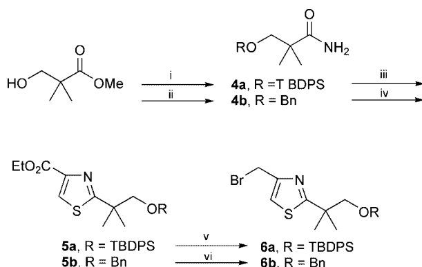
Scheme 2. Synthesis of the thiazole core. Reagents and conditions: (i): 1. TBDPSCl, imidazole, DMF, 95%; 2. KOH, EtOH, 80%; 3. \text{PCl}_5 , hexanes, then aq. \text{NH}_3 , 85%. (ii): 1. BnBr, NaH, 70%; 2. KOH, EtOH, 95%; 3. \text{PCl}_5 , hexanes, then aq. \text{NH}_3 , 90%. (iii): 1. Lawesson, DCM, 90%; 2. \text{BrCH}_2\text{COCO}_2\text{Et} , Py, TFAA, THF, 95%. (iv): 1. Lawesson, DCM, 95%; 2. \text{BrCH}_2\text{COCO}_2\text{Et} , EtOH, \Delta , 95%. (v): 1. DIBAL-H, \text{Et}_2\text{O} , -78^\circ\text{C} , 90%; 2. \text{CBr}_4 , \text{Ph}_3\text{P} , THF, 95%. (vi): 1. DIBAL-H, DCM, -40^\circ\text{C} , 80%; 2. \text{CBr}_4 , \text{Ph}_3\text{P} , THF, 80%.
