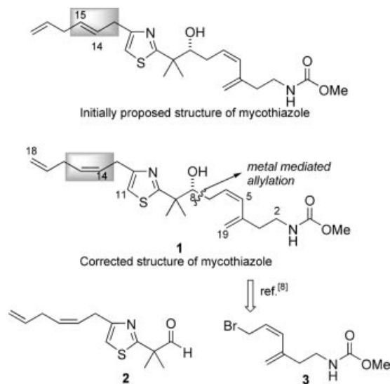
Scheme 1. Retrosynthetic analysis of mycothiazole.
