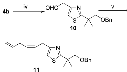
Scheme 3. Synthesis of C8–C18 fragments of mycOTHIAZOLE with a (Z)- \Delta^{14} configuration. Reagents and conditions: (i): \text{InCl}_3 , \equiv\text{MgBr} , \text{Pd}(\text{dppf})\text{Cl}_2 , THF, 70%. (ii): \text{CH}_2=\text{CHCH}_2\text{Br} , \text{EtMgBr} , CuBr, THF, 80%. (iii): \text{H}_2 ; Lindlar, quinoline, THF/EtOH, 26%. (iv): 1. Lawesson, DCM, 95%; 2. \text{ClCH}_2\text{COCH}_2\text{CO}_2\text{Et} , EtOH, \Delta , 95%; 3. DIBAL-H, PhMe, 95%. (v): \text{CH}_2=\text{CHCH}_2\text{CH}_2\text{PPh}_3\text{Br} , n\text{BuLi} , THF, 41%.
